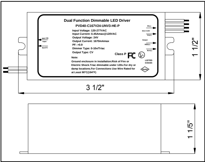
LED DRIVER DIAGRAM
